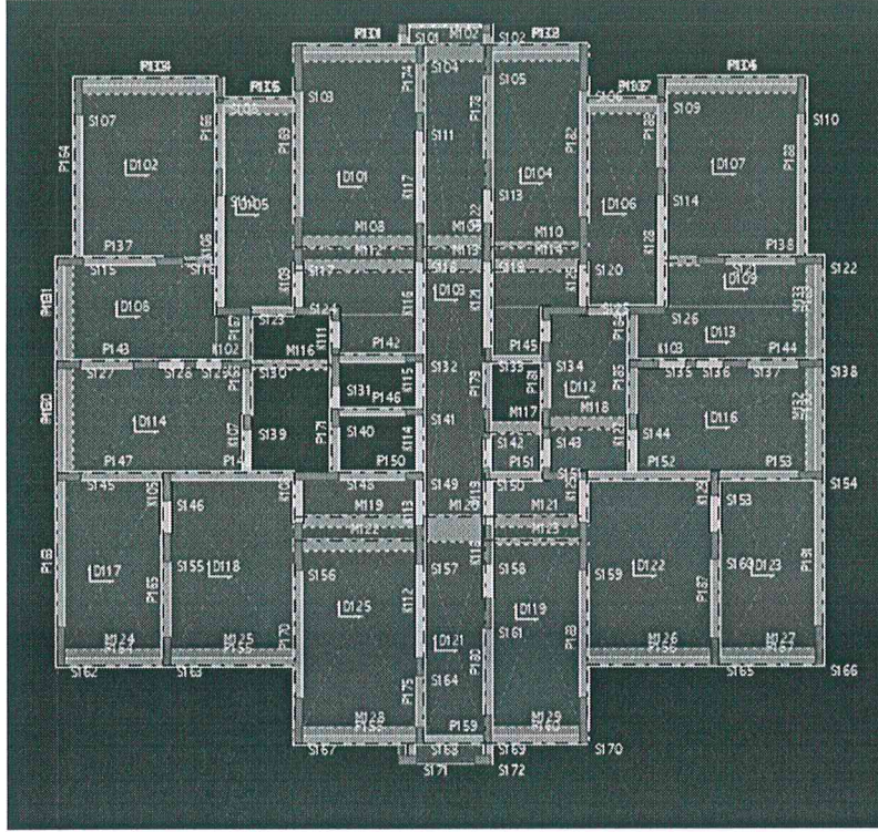
2. BODRUM KAT PLANI
